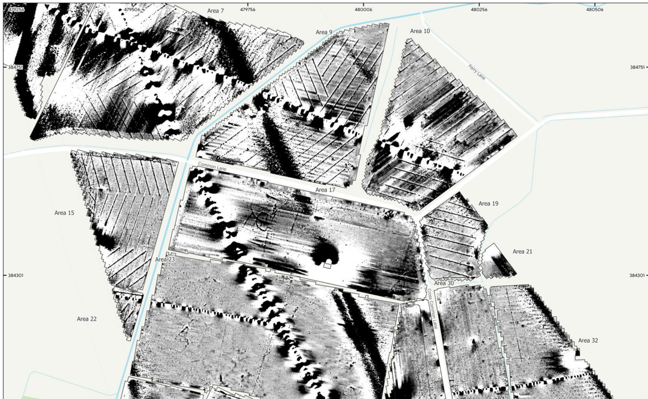
MSSK1773 - Steeple Solar, Nottinghamshire Figure 28 - Magnetic Total Field (Lower Sensors) (Areas 6, 7, 9, 10, 15, 17, 19, 21, 22, 23, 30, 31, 32, 33 & 34) 1:3,500 @ A3 © Magnitude Surveys 2025 Contains Ordnance Survey data © Crown Copyright and database right 2025
