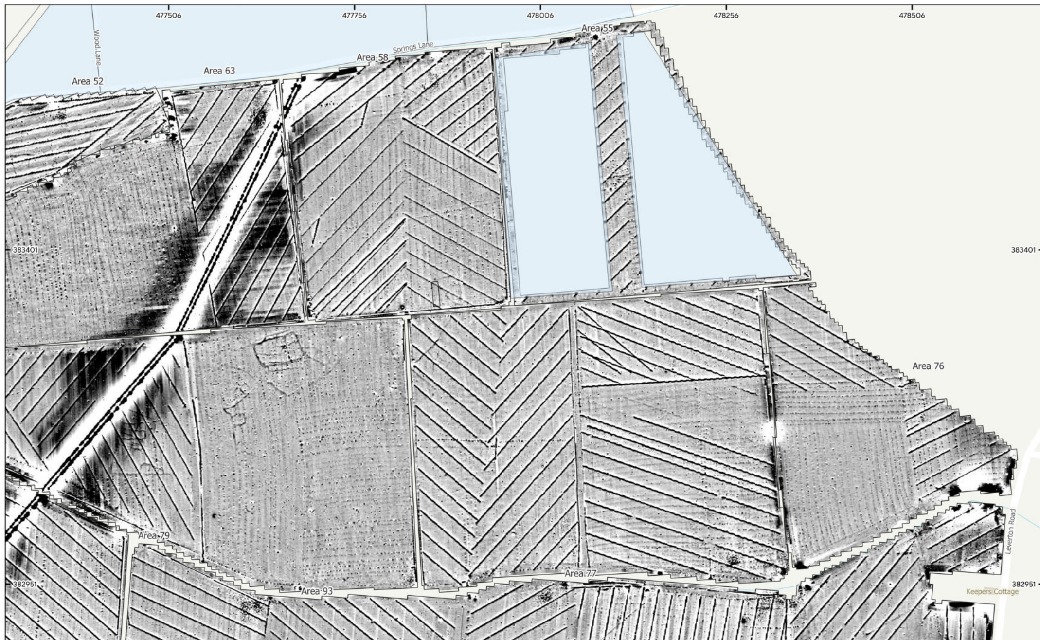
MSSK1773 - Steeple Solar, Nottinghamshire Figure 13 - Magnetic Total Field (Lower Sensors) (Areas 52, 55, 58, 63, 76, 77, 79, 89 & 93) 1:3,500 @ A3 © Magnitude Surveys 2025 Contains Ordnance Survey data © Crown Copyright and database right 2025
