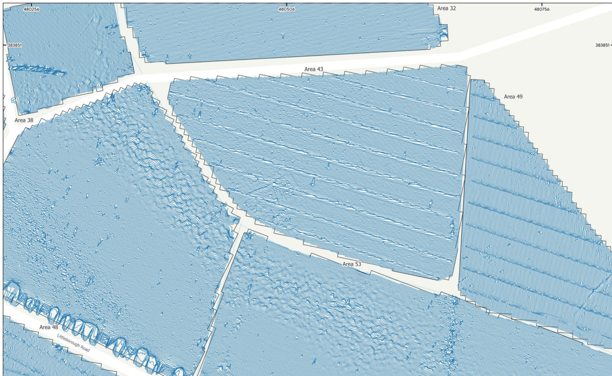
MSSK1773 - Steeple Solar, Nottinghamshire Figure 50 - XY Trace Plot (Area of Archaeological Activity 3) 30nT/cm at 1:1,500 @ A3 © Magnitude Surveys 2025 Contains Ordnance Survey data © Crown Copyright and database right 2025
