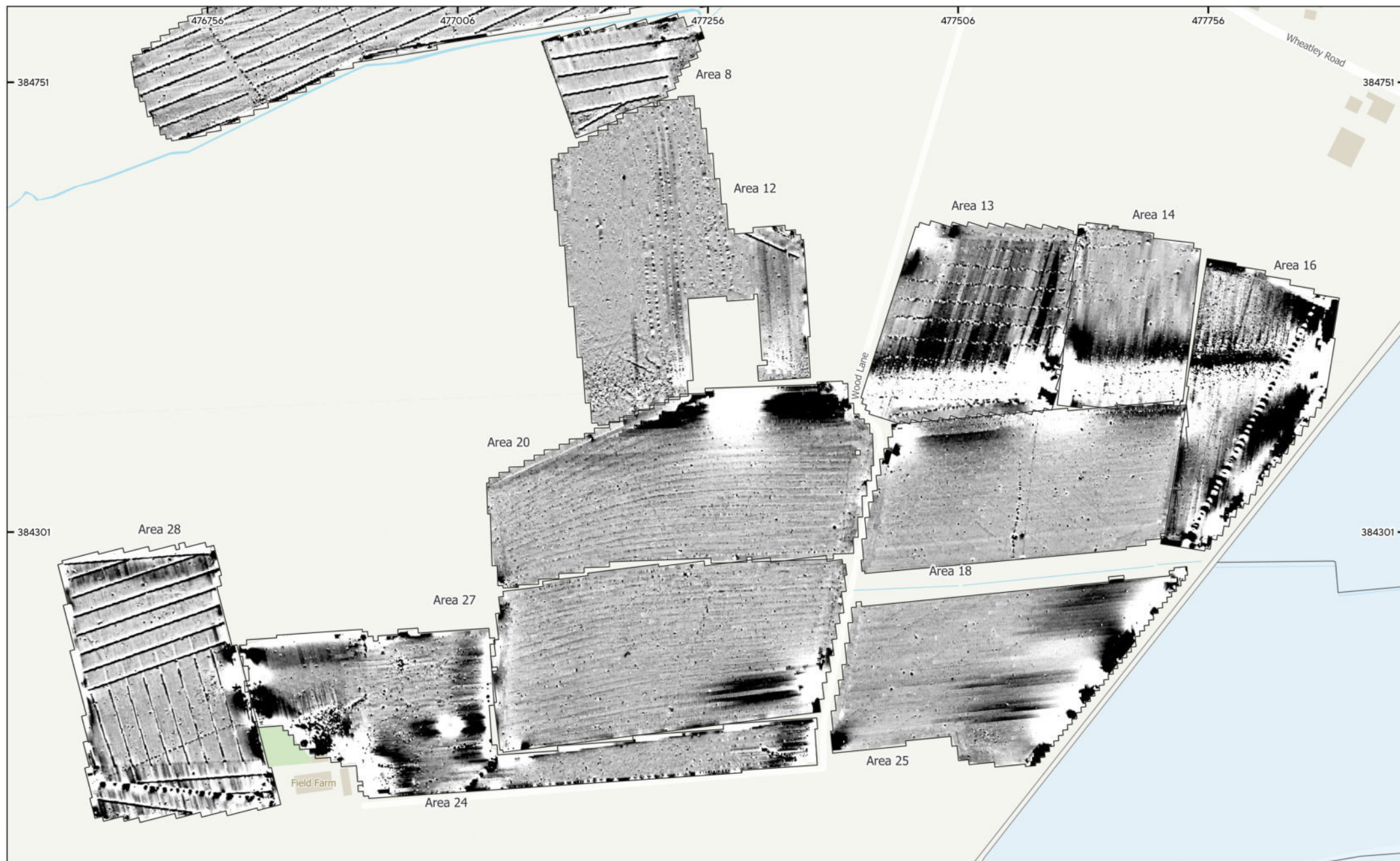
MSSK1773 - Steeple Solar, Nottinghamshire Figure 7 - Magnetic Total Field (Lower Sensors) (Areas 12, 13, 14, 16, 18, 20, 24, 25, 27 & 28) 1:3,500 @ A3 © Magnitude Surveys 2025 Contains Ordnance Survey data © Crown Copyright and database right 2025
