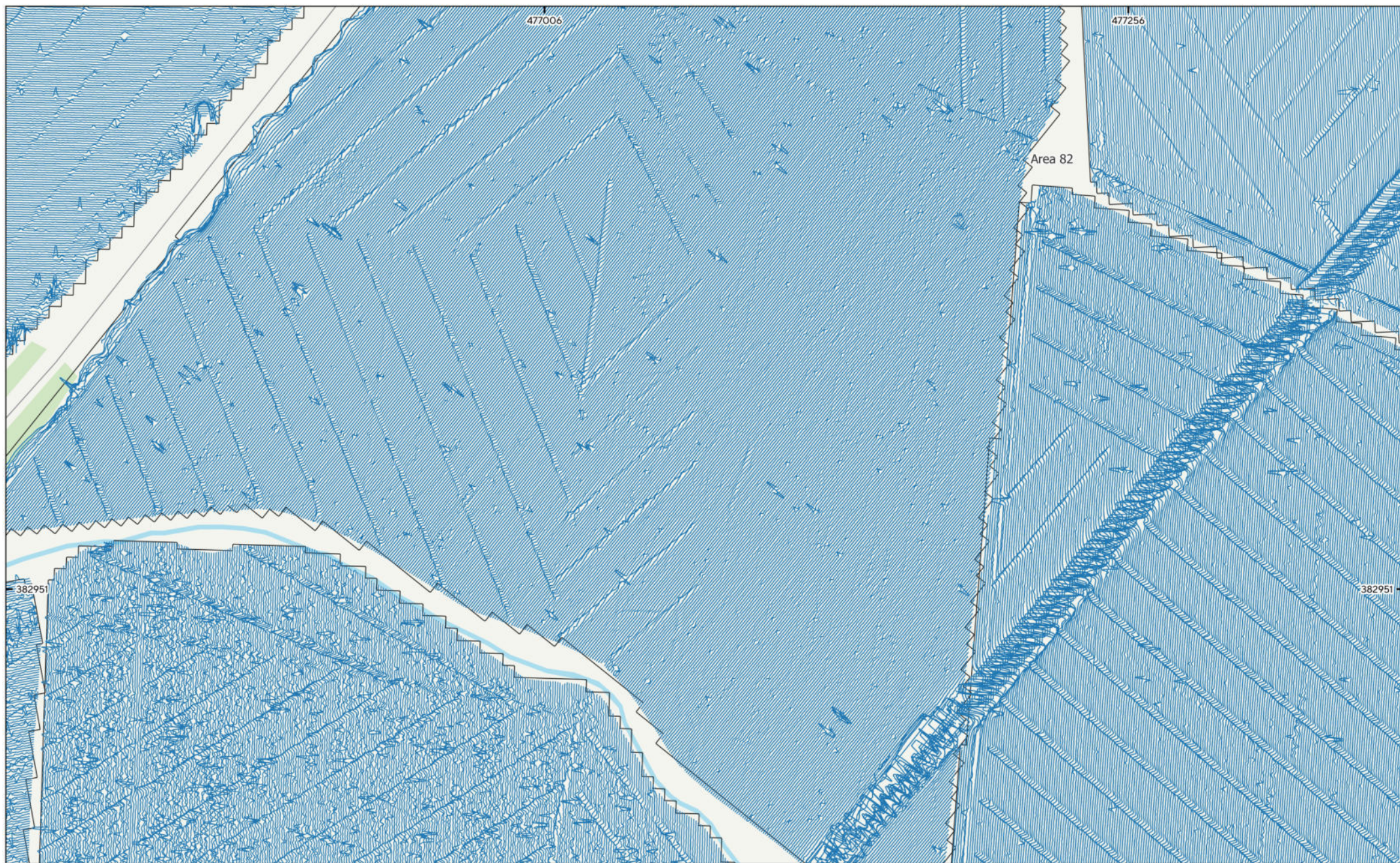
MSSK1773 - Steeple Solar, Nottinghamshire Figure 56 - XY Trace Plot (Area of Archaeological Activity 5) 30nT/cm at 1:1,500 @ A3 © Magnitude Surveys 2025 Contains Ordnance Survey data © Crown Copyright and database right 2025
