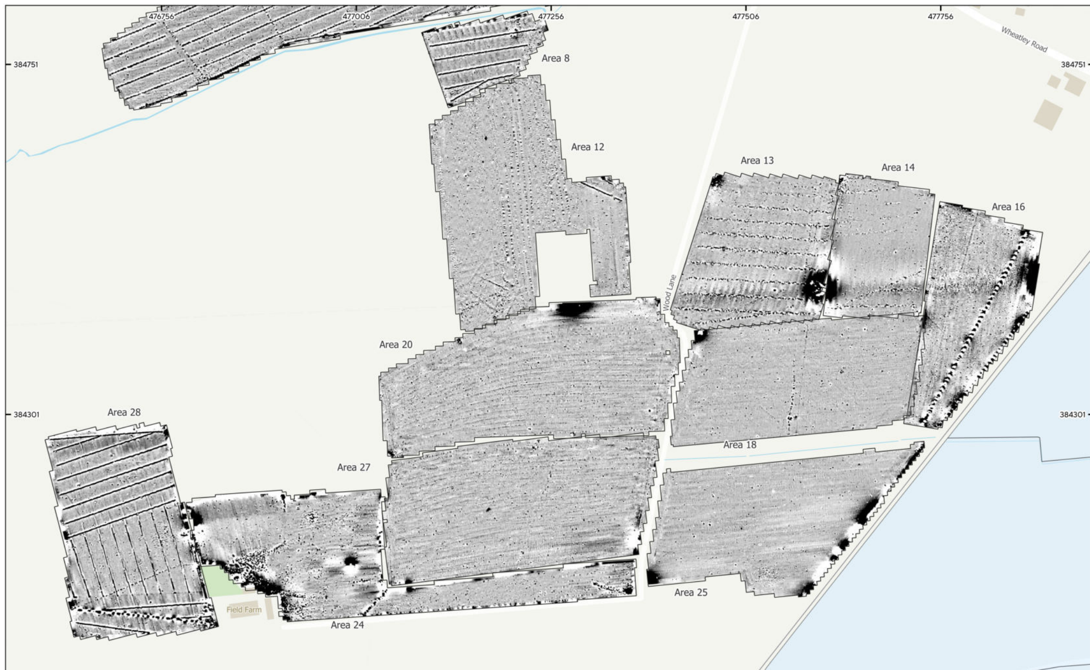
MSSK1773 - Steeple Solar, Nottinghamshire Figure 6 - Magnetic Gradient (Areas 12, 13, 14, 16, 18, 20, 24, 25, 27 & 28) 1:3,500 @ A3 © Magnitude Surveys 2025 Contains Ordnance Survey data © Crown Copyright and database right 2025
