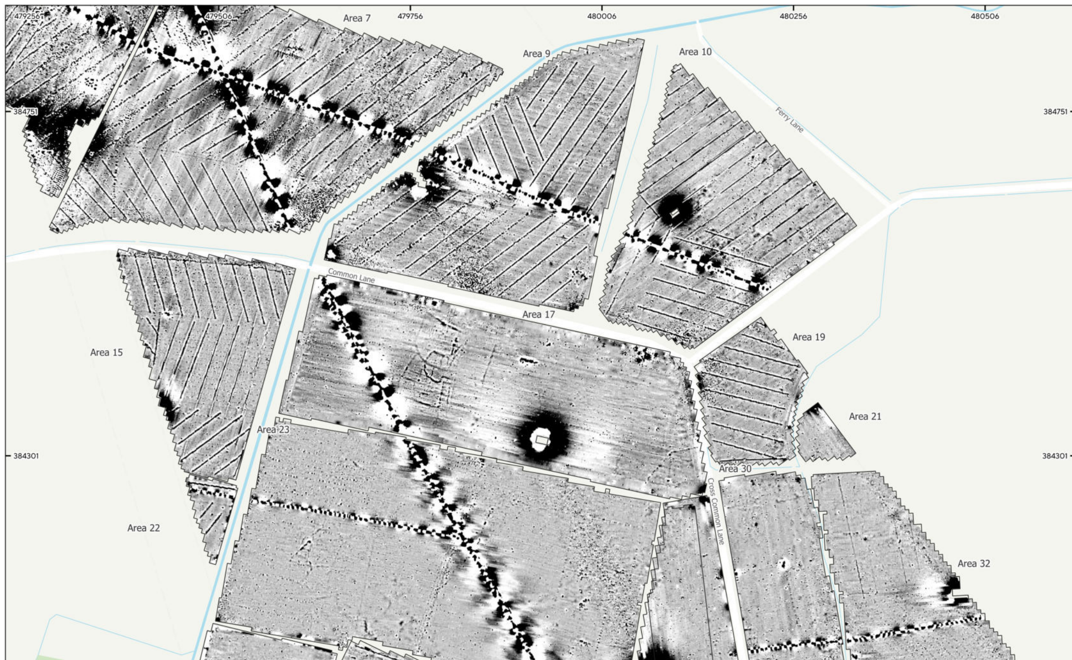
MSSK1773 - Steeple Solar, Nottinghamshire Figure 27 - Magnetic Gradient (Areas 6, 7, 9, 10, 15, 17, 19, 21, 22, 23, 30, 31, 32, 33 & 34) 1:3,500 @ A3 © Magnitude Surveys 2025 Contains Ordnance Survey data © Crown Copyright and database right 2025
