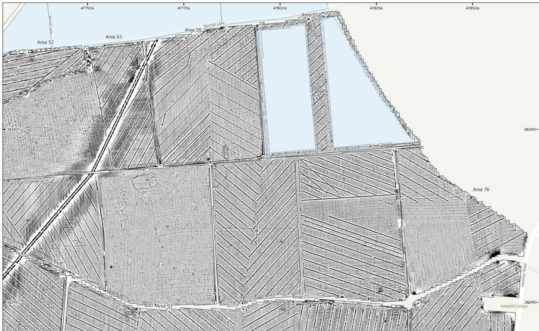
MSSK1773 - Steeple Solar, Nottinghamshire Figure 12 - Magnetic Gradient (Areas 52, 55, 58, 63, 76, 77, 79, 89 & 93) 1:3,500 @ A3 © Magnitude Surveys 2025 Contains Ordnance Survey data © Crown Copyright and database right 2025
