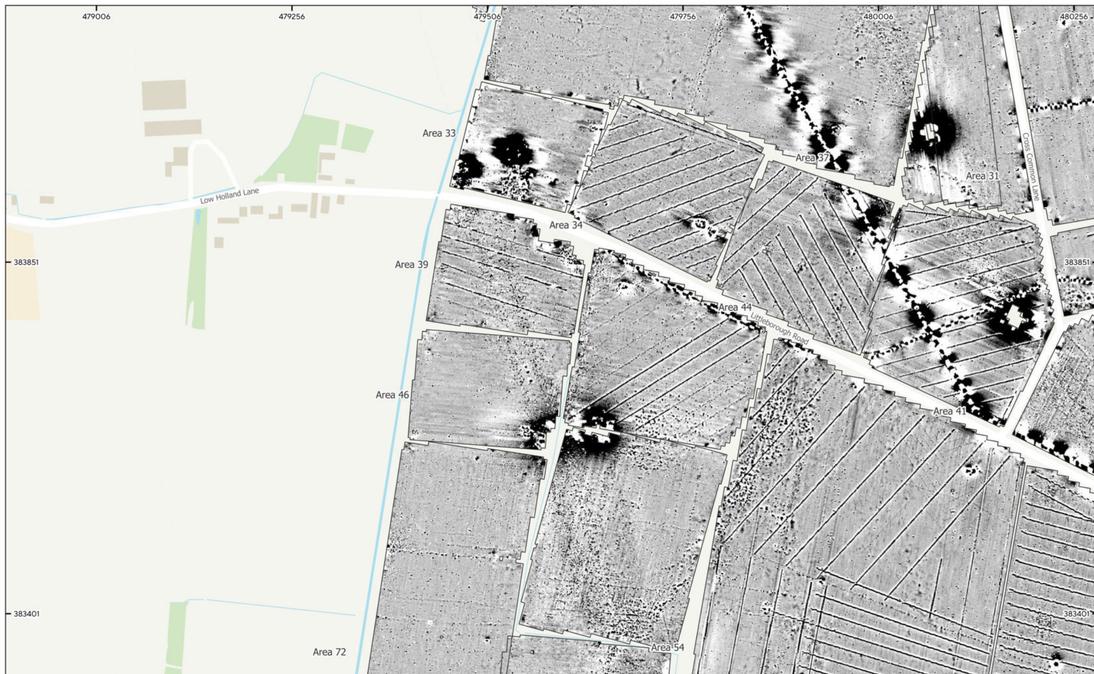
MSSK1773 - Steeple Solar, Nottinghamshire Figure 30 - Magnetic Gradient (Areas 22, 34, 30, 31, 33, 34, 37, 38, 39, 41, 44, 46, 48, 54, 62, 66, 69 & 72) 1:3,500 @ A3 © Magnitude Surveys 2025 Contains Ordnance Survey data © Crown Copyright and database right 2025
