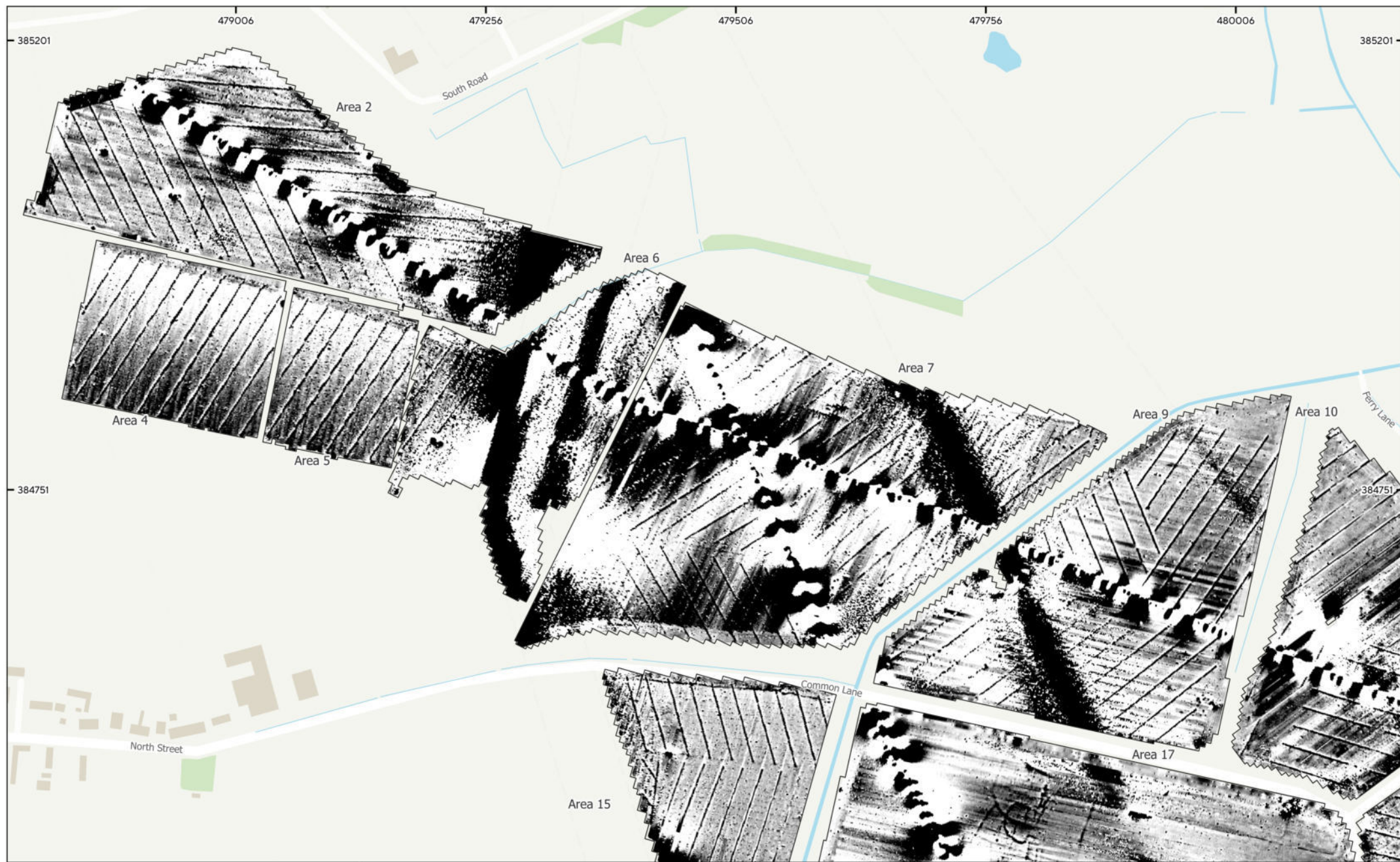
MSSK1773 - Steeple Solar, Nottinghamshire Figure 25 - Magnetic Total Field (Lower Sensors) (Areas 2, 4, 5, 6, 7, 9, 10, 15, 17 & 19) 1:3,500 @ A3 © Magnitude Surveys 2025 Contains Ordnance Survey data © Crown Copyright and database right 2025
