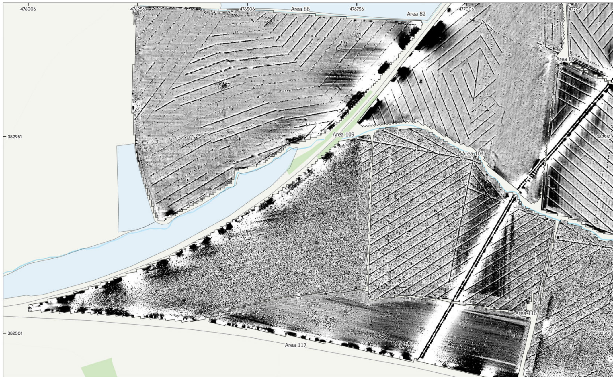
MSSK1773 - Steeple Solar, Nottinghamshire Figure 16 - Magnetic Total Field (Lower Sensors) (Areas 79, 82, 86, 89, 104, 109, 116 & 117) 1:3,500 @ A3 © Magnitude Surveys 2025 Contains Ordnance Survey data © Crown Copyright and database right 2025
