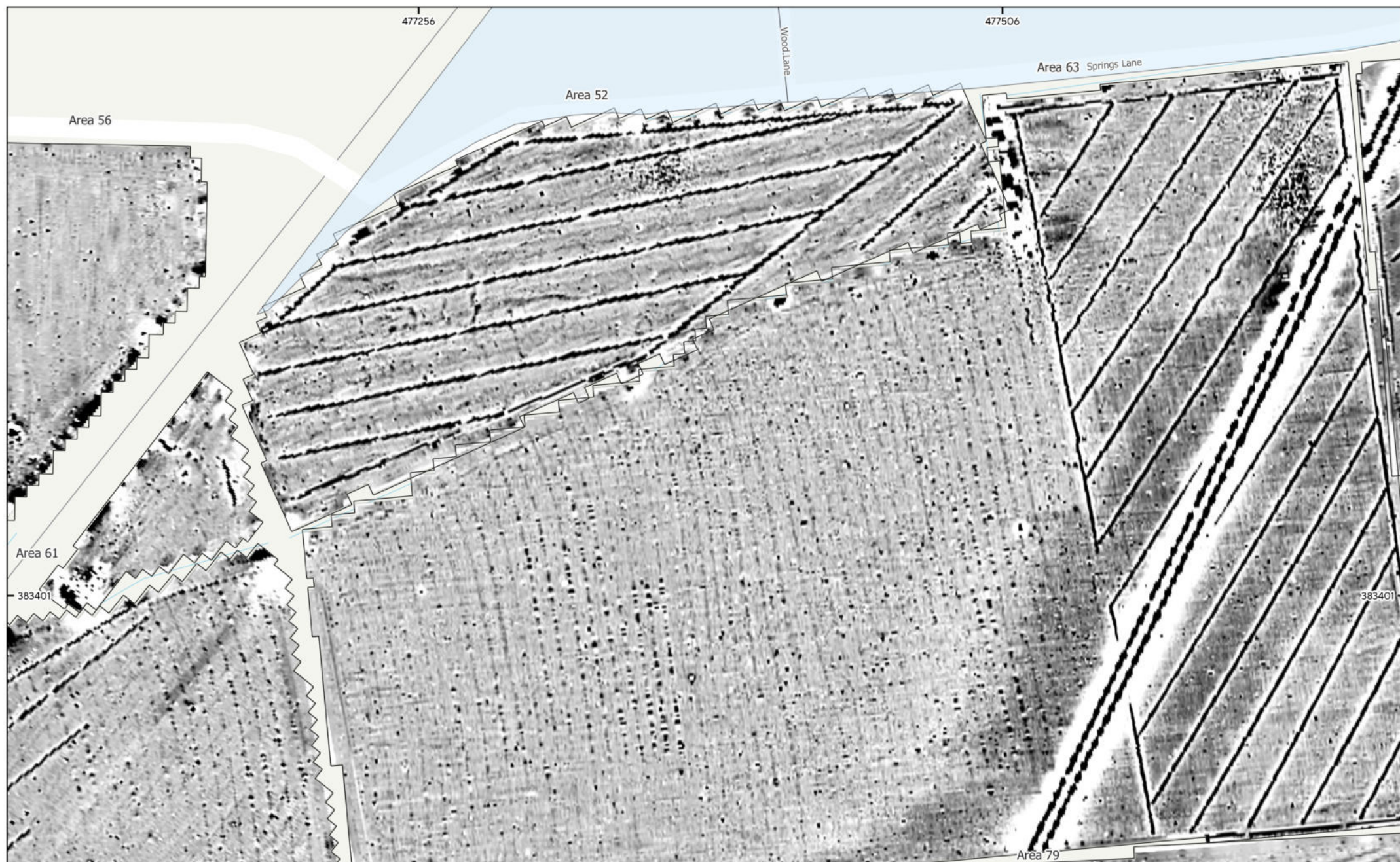
MSSK1773 - Steeple Solar, Nottinghamshire Figure 60 - Magnetic Gradient (Area of Archaeological Activity 7) 1:1,500 @ A3 © Magnitude Surveys 2025 Contains Ordnance Survey data © Crown Copyright and database right 2025
