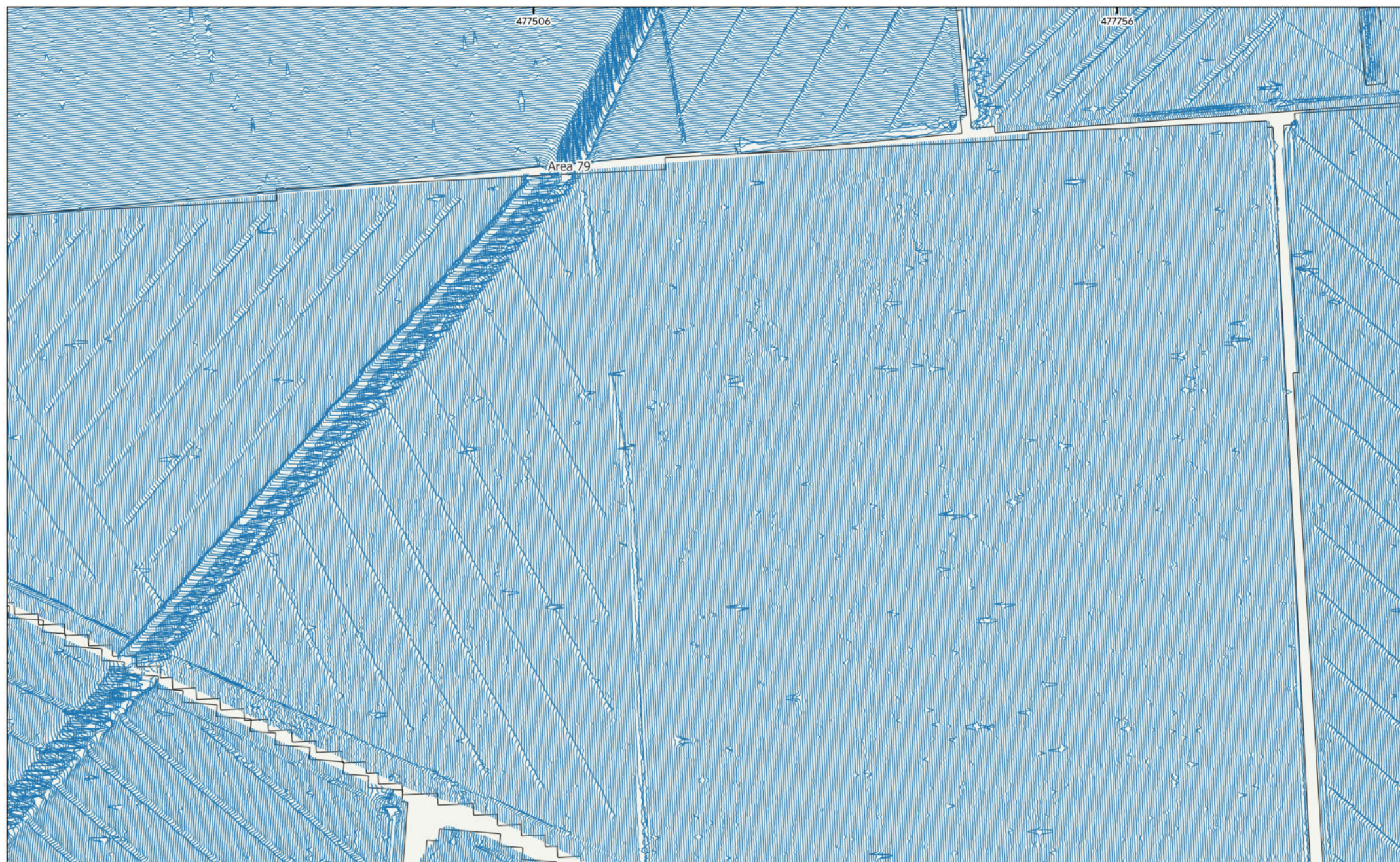
MSSK1773 - Steeple Solar, Nottinghamshire Figure 59 - XY Trace Plot (Area of Archaeological Activity 6) 30nT/cm at 1:1,500 @ A3 © Magnitude Surveys 2025 Contains Ordnance Survey data © Crown Copyright and database right 2025
