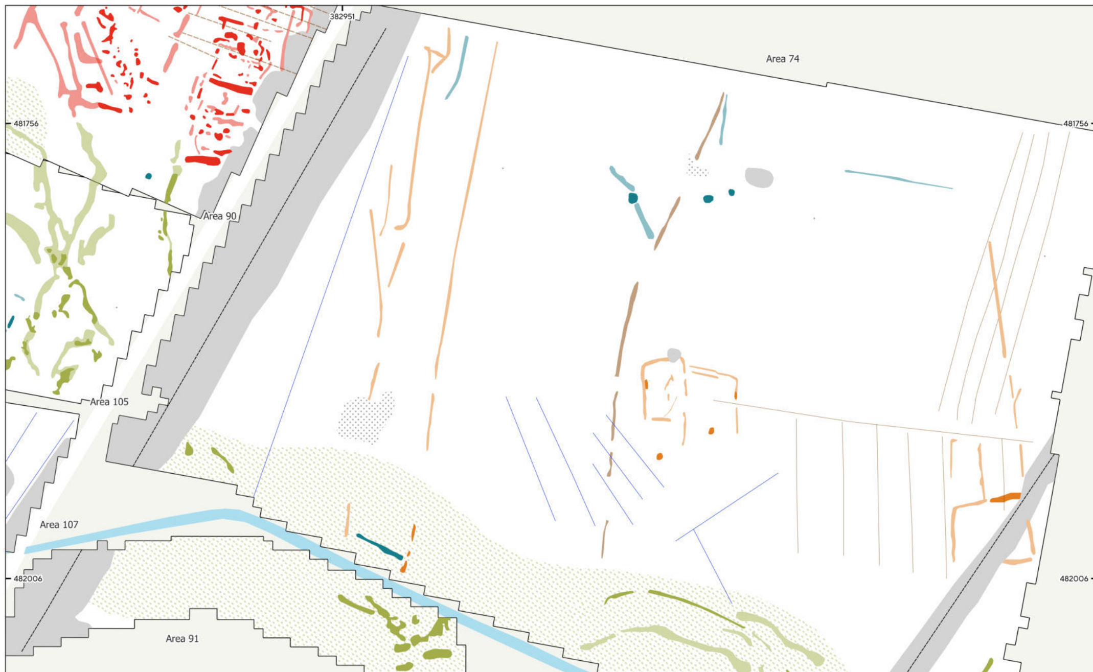
MSSK1773 - Steeple Solar, Nottinghamshire Figure 46 - Magnetic Interpretation (Area of Archaeological Activity 2) 1:1,500 @ A3 © Magnitude Surveys 2025 Contains Ordnance Survey data © Crown Copyright and database right 2025
