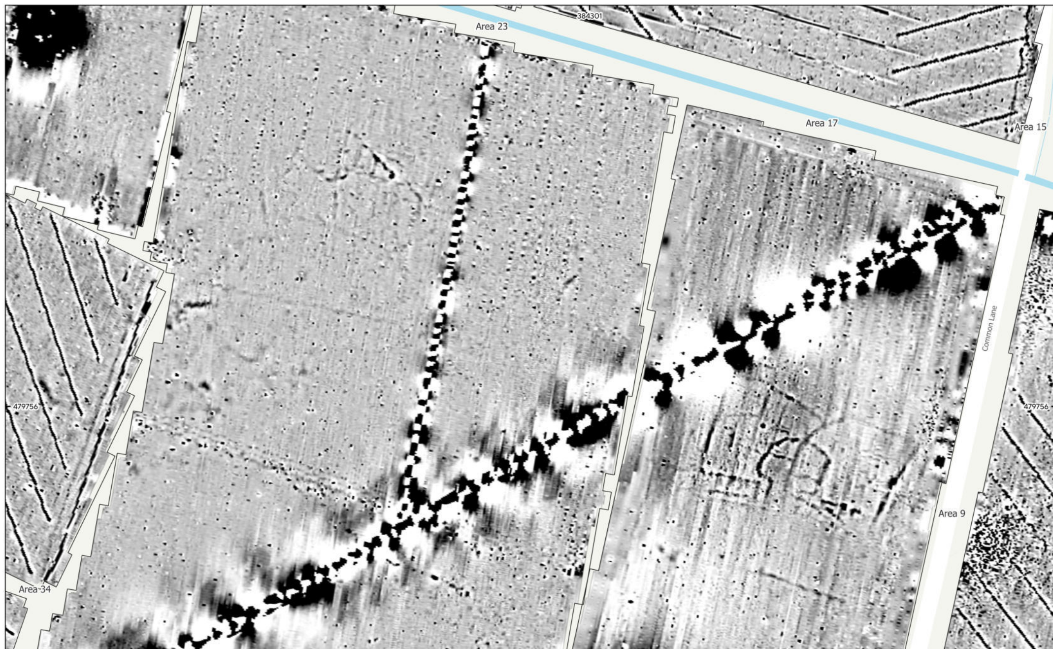
MSSK1773 - Steeple Solar, Nottinghamshire Figure 51 - Magnetic Gradient (Area of Archaeological Activity 4) 1:1,500 @ A3 © Magnitude Surveys 2025 Contains Ordnance Survey data © Crown Copyright and database right 2025
