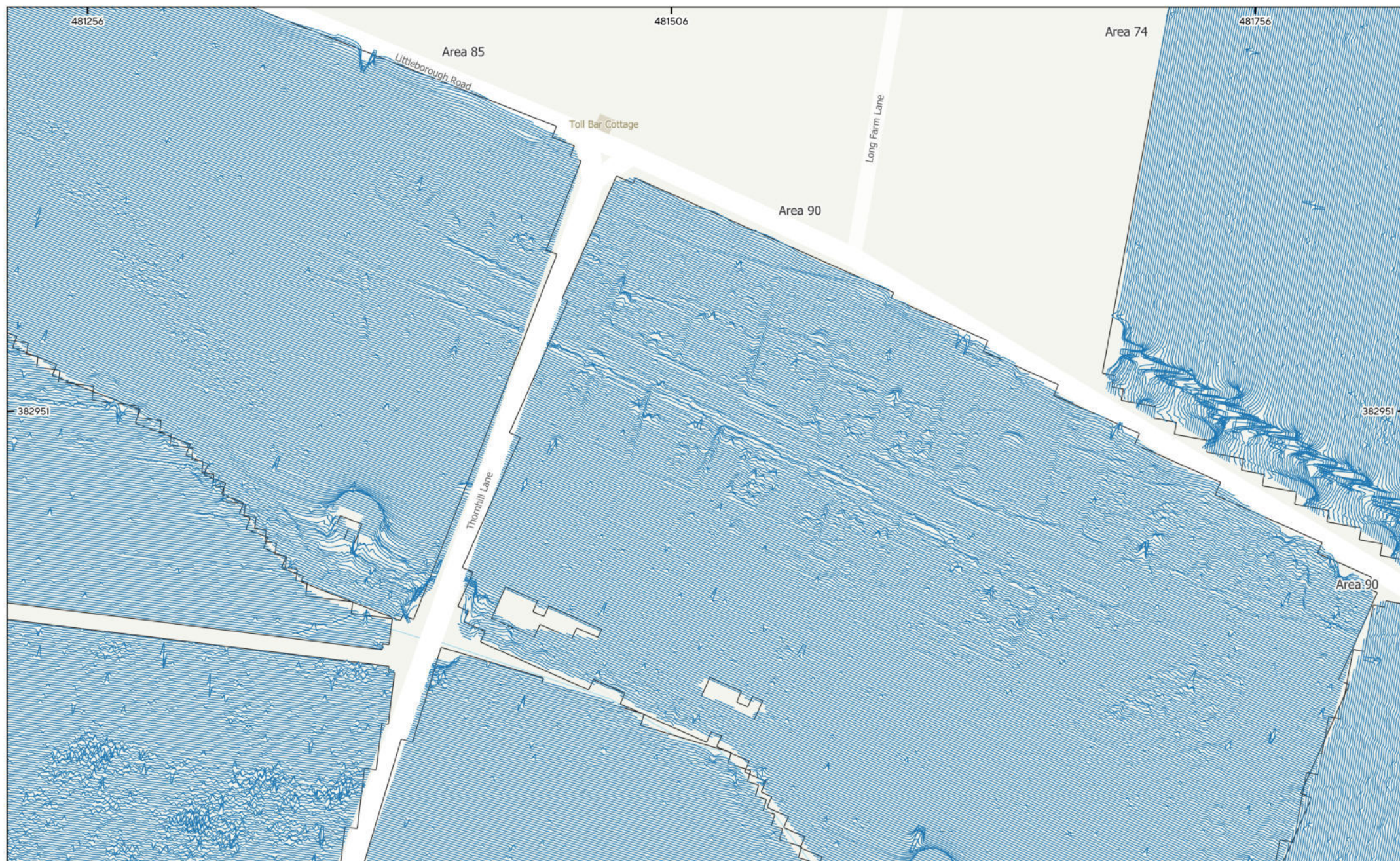
MSSK1773 - Steeple Solar, Nottinghamshire Figure 44 - XY Trace Plot (Area of Archaeological Activity 1) 30nT/cm at 1:1,500 @ A3 © Magnitude Surveys 2025 Contains Ordnance Survey data © Crown Copyright and database right 2025
