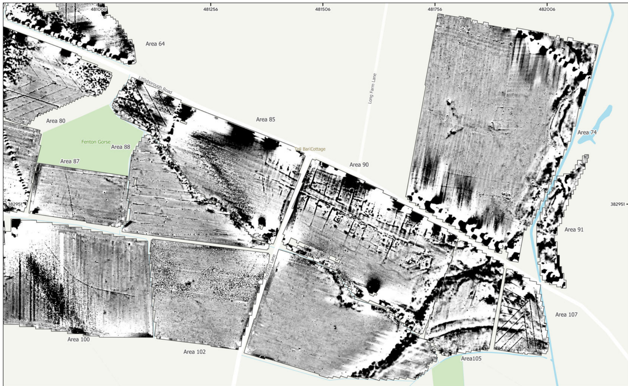
MSSK1773 - Steeple Solar, Nottinghamshire Figure 40 - Magnetic Total Field (Lower Sensors) (Areas 64, 74, 80, 85, 87, 88, 90, 91, 94, 100, 102, 105, 107 & 111) 1:3,500 @ A3 © Magnitude Surveys 2025 Contains Ordnance Survey data © Crown Copyright and database right 2025
