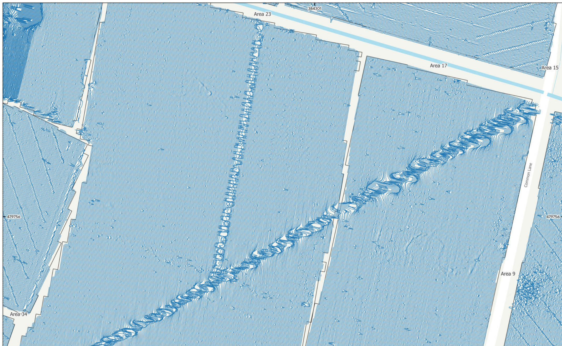
MSSK1773 - Steeple Solar, Nottinghamshire Figure 53 - XY Trace Plot (Area of Archaeological Activity 4) 30nT/cm at 1:1,500 @ A3 © Magnitude Surveys 2025 Contains Ordnance Survey data © Crown Copyright and database right 2025
