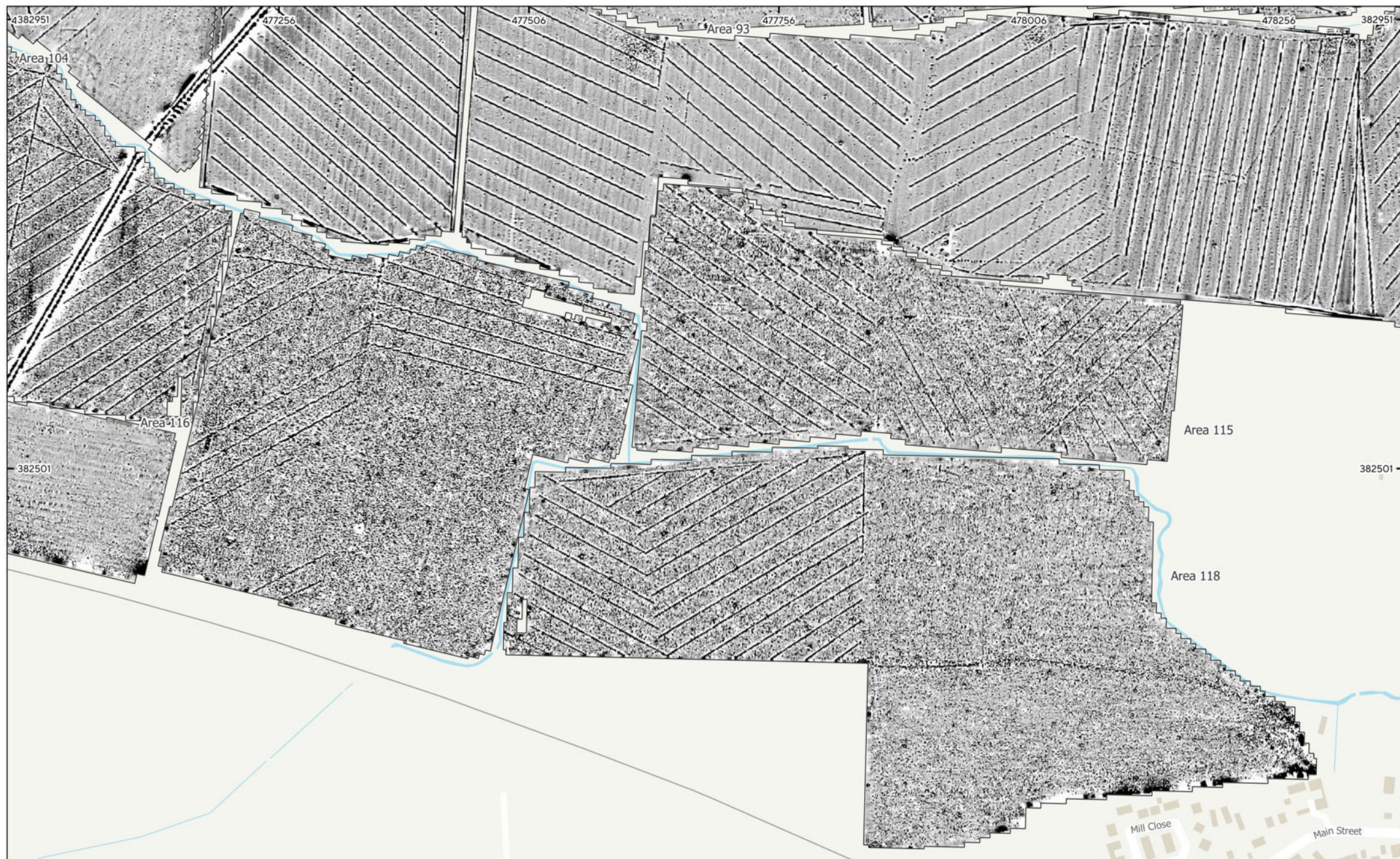
MSSK1773 - Steeple Solar, Nottinghamshire Figure 18 - Magnetic Gradient (Areas 77, 79, 82, 89, 93, 104, 115, 116, 117 & 118) 1:3,500 @ A3 © Magnitude Surveys 2025 Contains Ordnance Survey data © Crown Copyright and database right 2025
