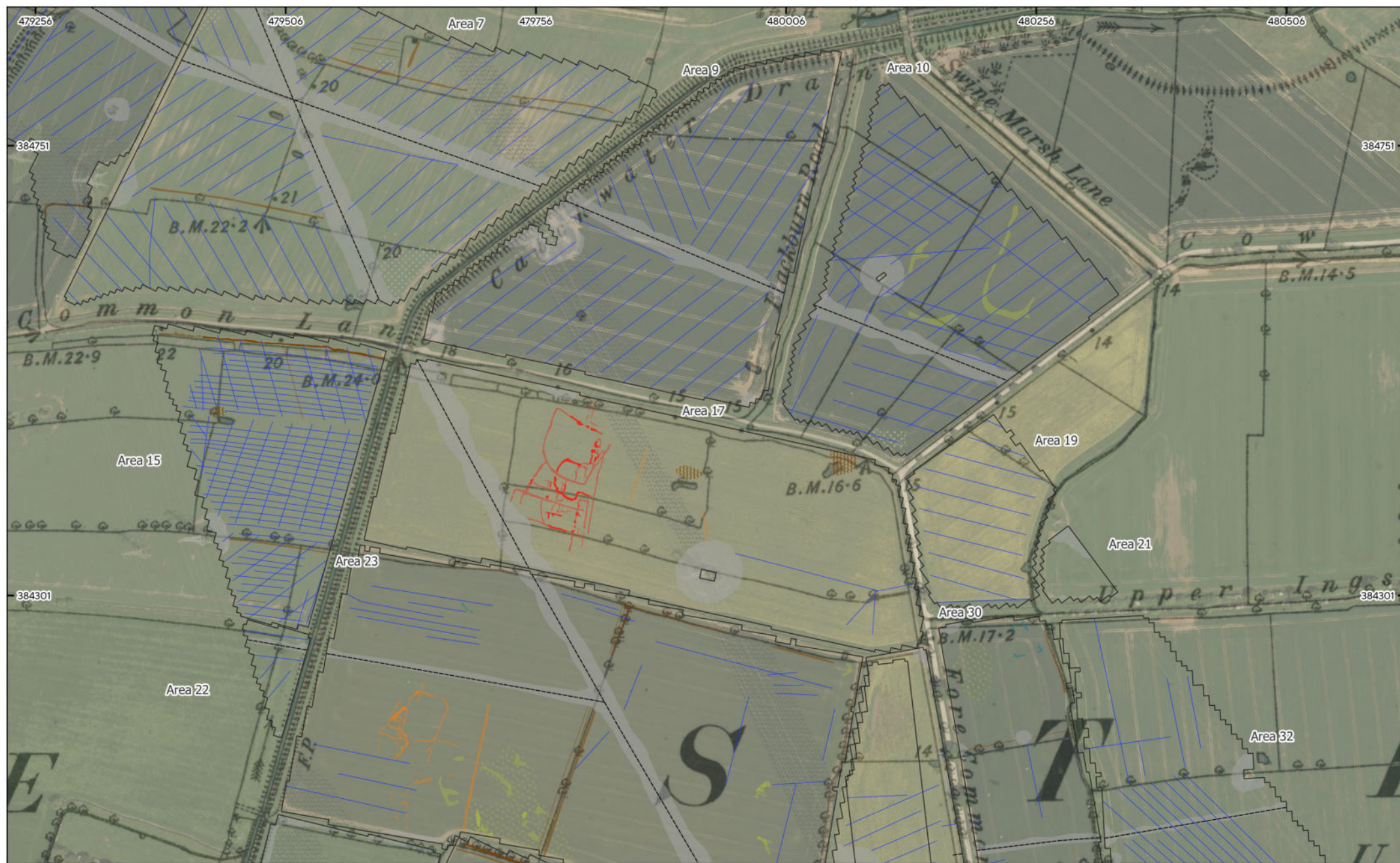
MSSK1773 - Steeple Solar, Nottinghamshire Figure 29 - Magnetic Interpretation over Historical Mapping and Satellite Imagery (Areas 6, 7, 9, 10, 15, 17, 19, 21, 22, 23, 30, 31, 32, 33 & 34) 1:3,500 @ A3 © Magnitude Surveys 2025 Contains historical mapping © CLS Data 2025 Ordnance Survey, 6" 2nd edition c. 1882-1913 Contains satellite imagery © Bing Satellite 2025
