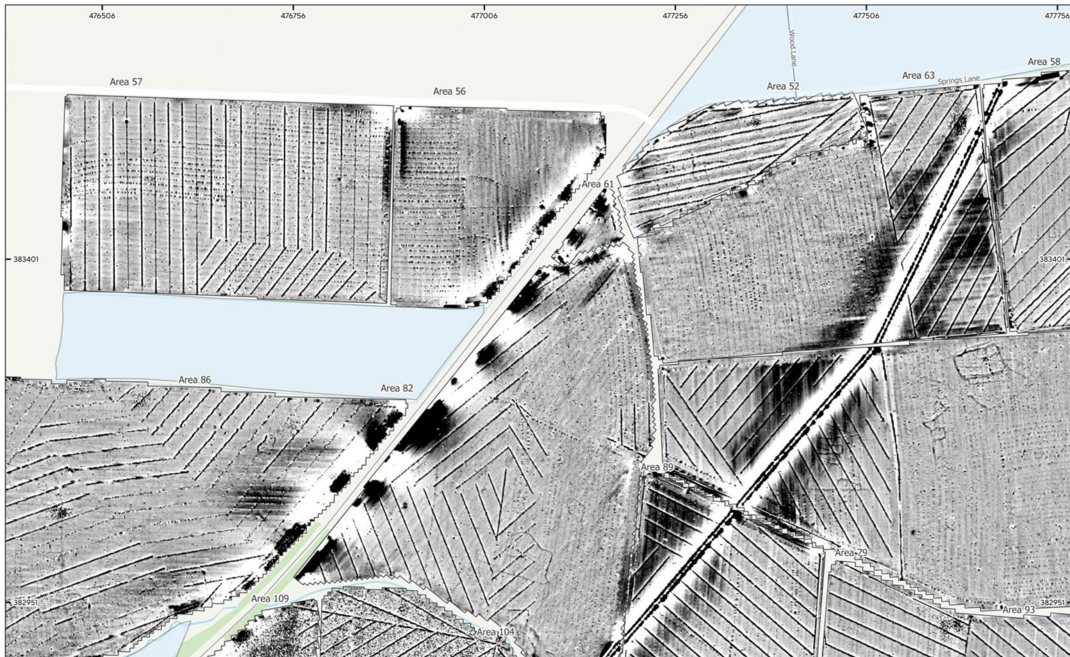
MSSK1773 - Steeple Solar, Nottinghamshire Figure 10 - Magnetic Total Field (Lower Sensors) (Areas 52, 56, 57, 58, 61, 63, 79, 82, 86, 89, 93, 104 & 109) 1:3,500 @ A3 © Magnitude Surveys 2025 Contains Ordnance Survey data © Crown Copyright and database right 2025
